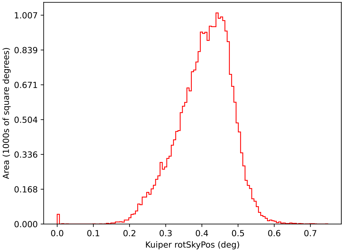
too_elab_r32_d2_griz_v3.4_10yrs i: Kuiper rotSkyPos
