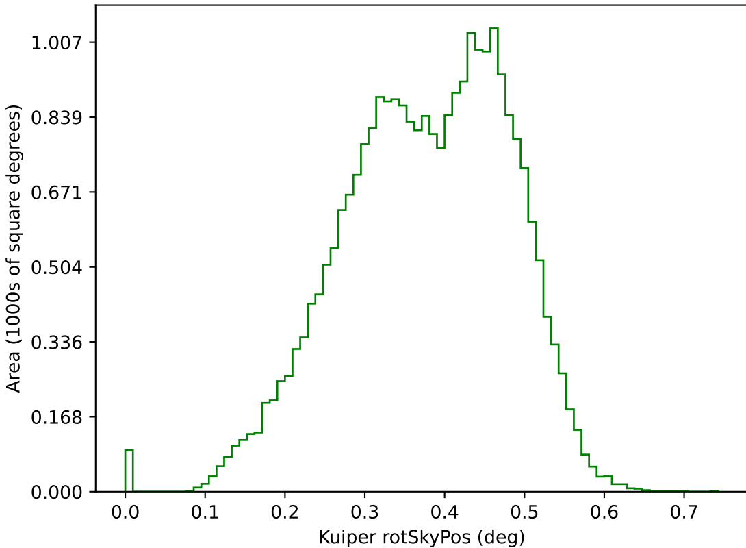
too_elab_r32_d2_griz_v3.4_10yrs g: Kuiper rotSkyPos
