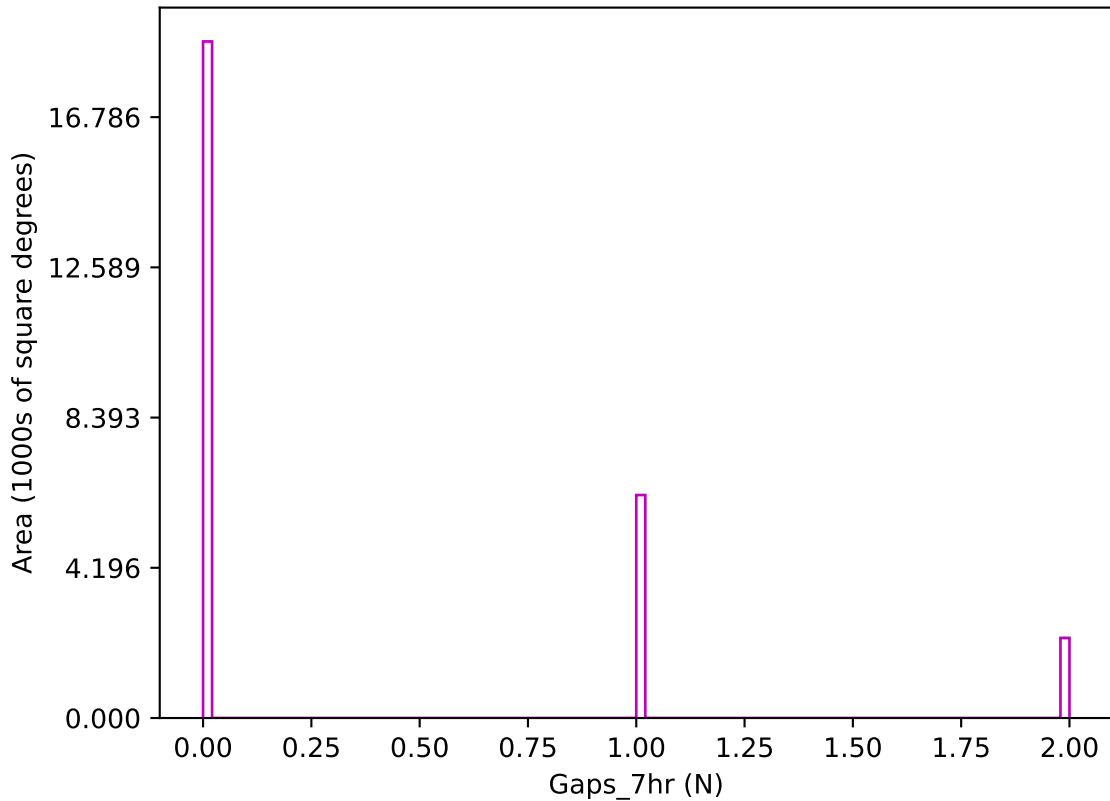
too_elab_r32_d2_griz_v3.4_10yrs z band: Gaps_7hr
