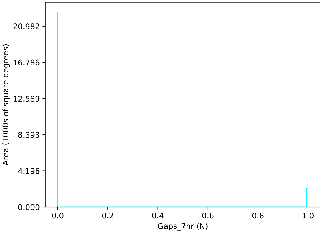
too_elab_r32_d2_griz_v3.4_10yrs u band: Gaps_7hr
