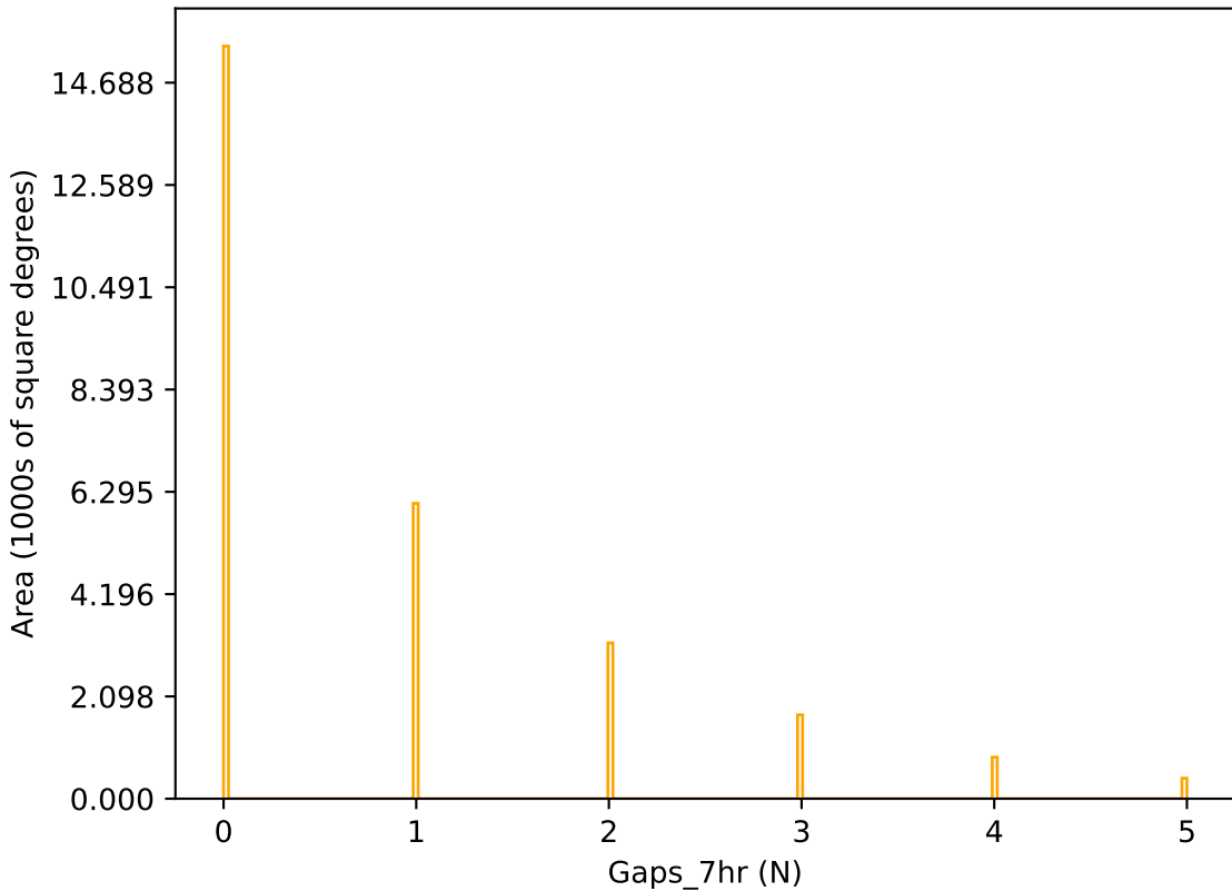
too_elab_r32_d2_griz_v3.4_10yrs r band: Gaps_7hr
