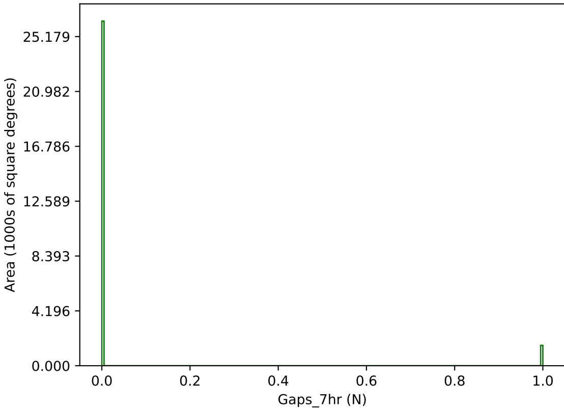
too_elab_r32_d2_griz_v3.4_10yrs g band: Gaps_7hr
