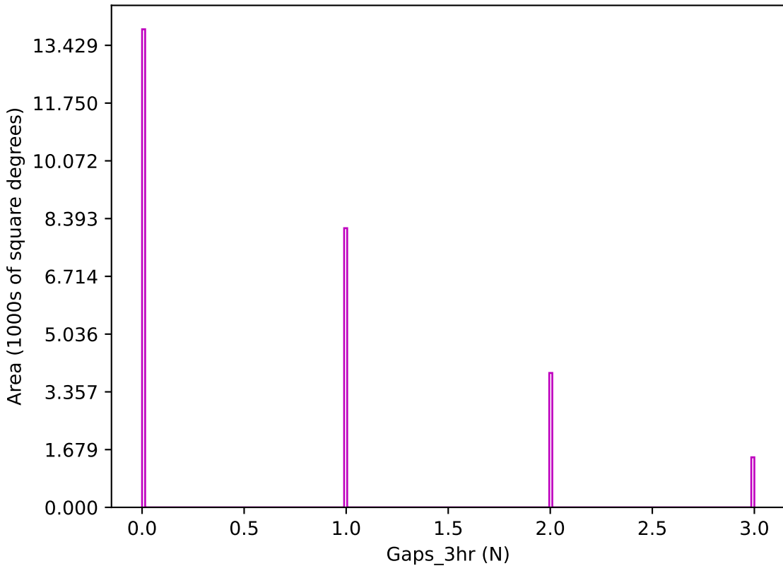
too_elab_r32_d2_griz_v3.4_10yrs z band: Gaps_3hr
