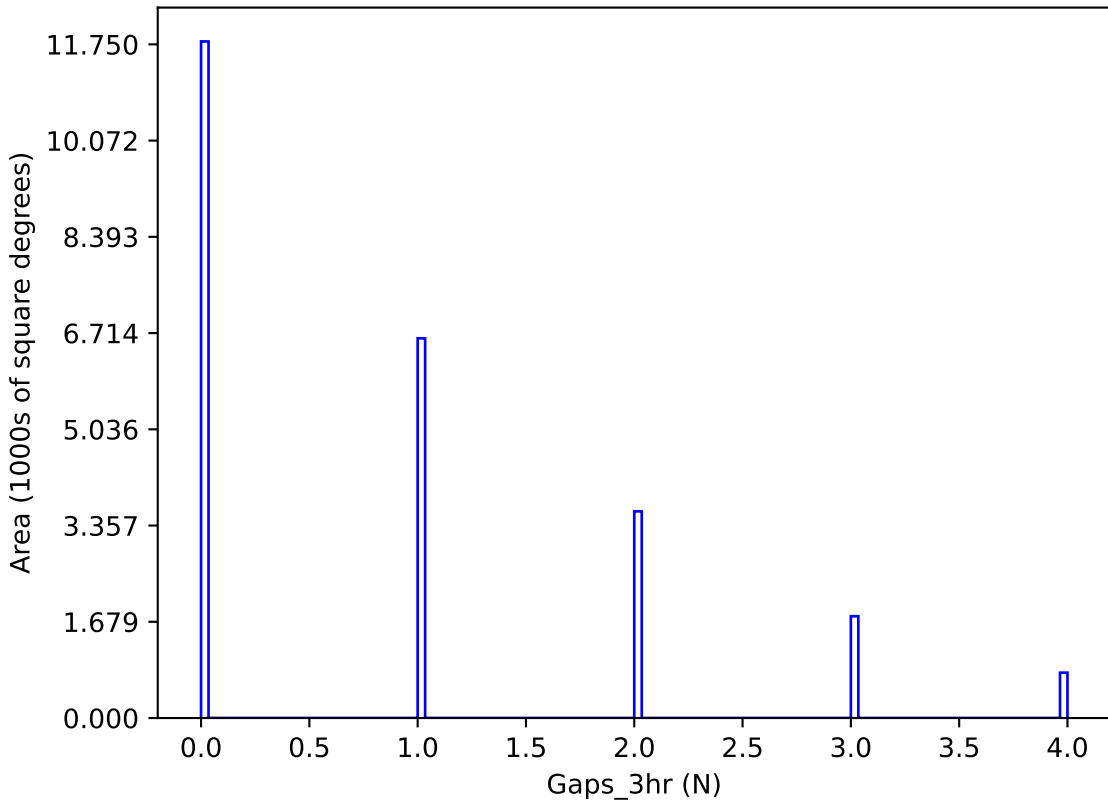
too_elab_r32_d2_griz_v3.4_10yrs y band: Gaps_3hr
