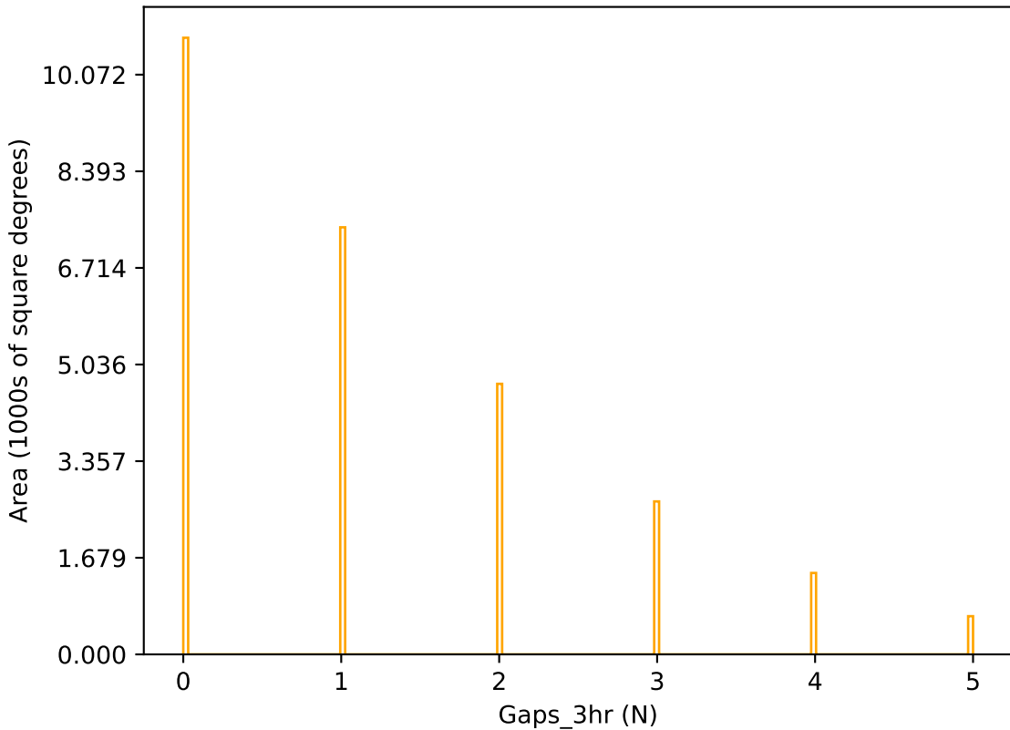
too_elab_r32_d2_griz_v3.4_10yrs r band: Gaps_3hr
