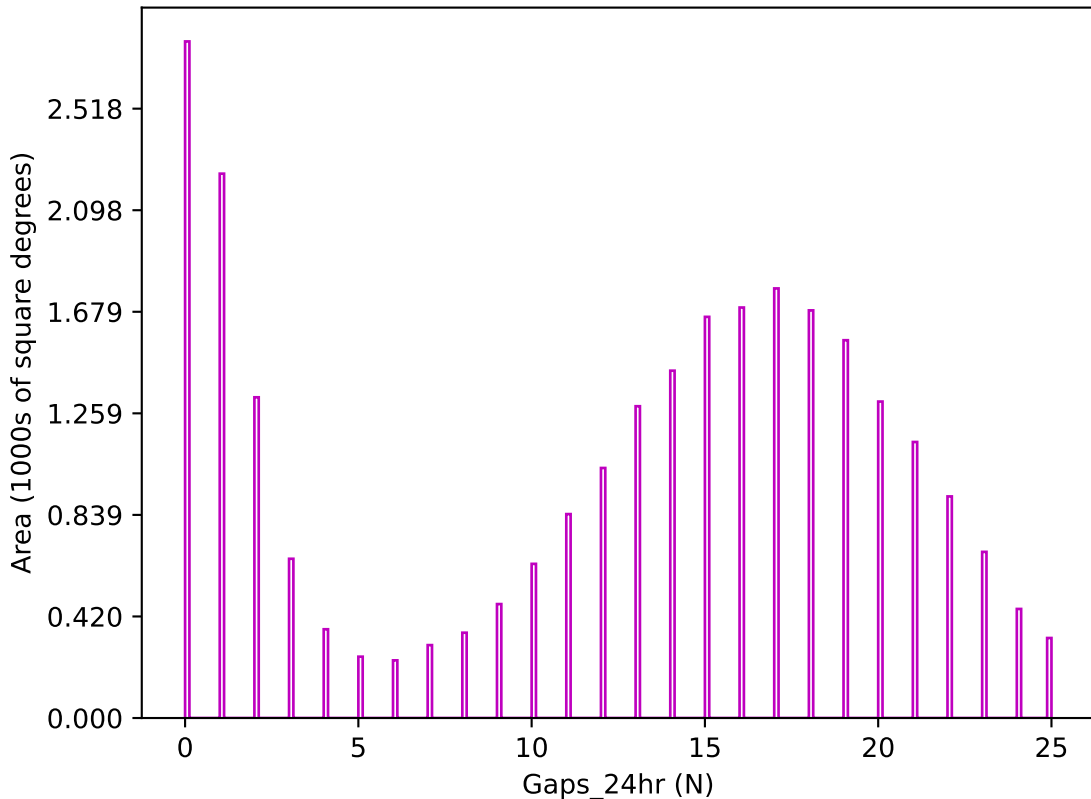
too_elab_r32_d2_griz_v3.4_10yrs z band: Gaps_24hr
