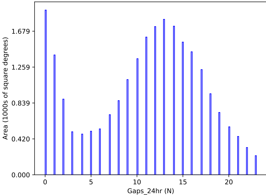
too_elab_r32_d2_griz_v3.4_10yrs y band: Gaps_24hr
