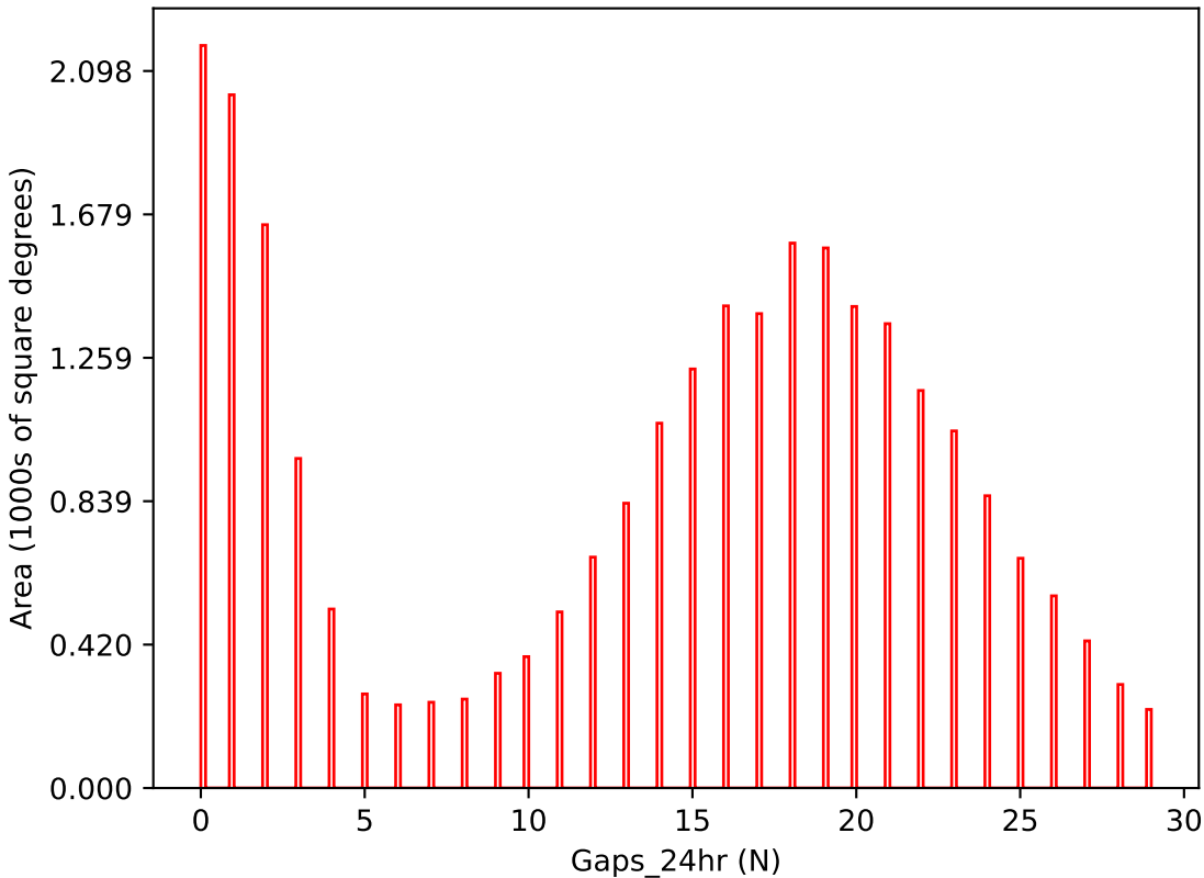
too_elab_r32_d2_griz_v3.4_10yrs i band: Gaps_24hr
