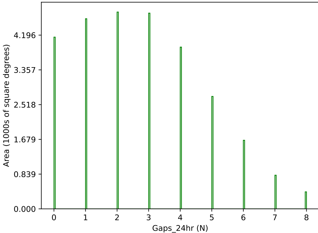
too_elab_r32_d2_griz_v3.4_10yrs g band: Gaps_24hr
