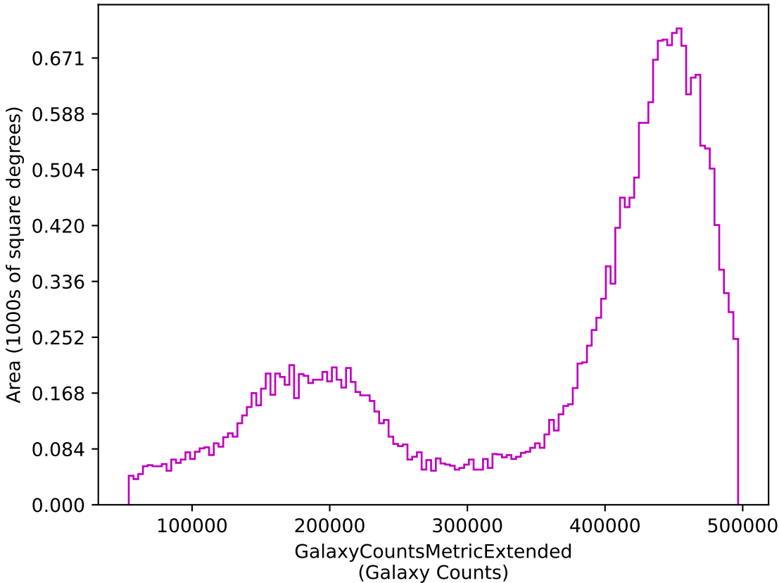
too_elab_r32_d2_griz_v3.4_10yrs z: GalaxyCountsMetricExtended
