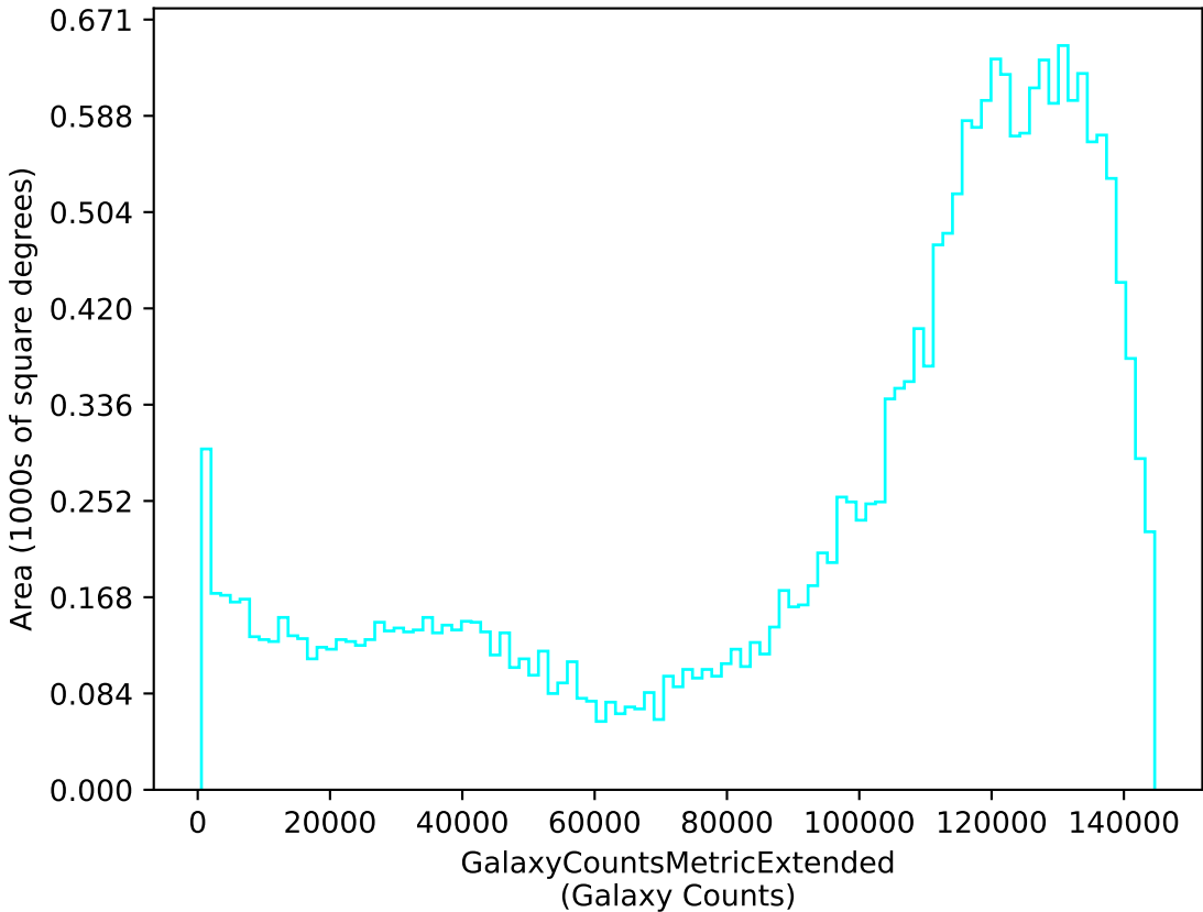
too_elab_r32_d2_griz_v3.4_10yrs u: GalaxyCountsMetricExtended
