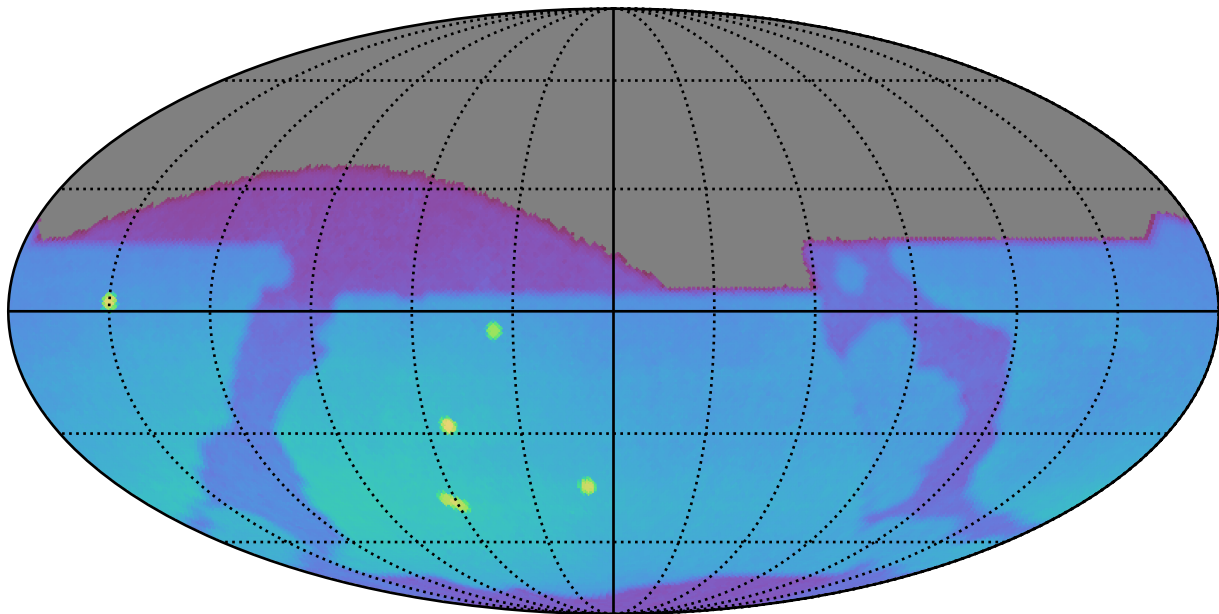
too_elab_r32_d2_griz_v3.4_10yrs : Brown Dwarf, L4
