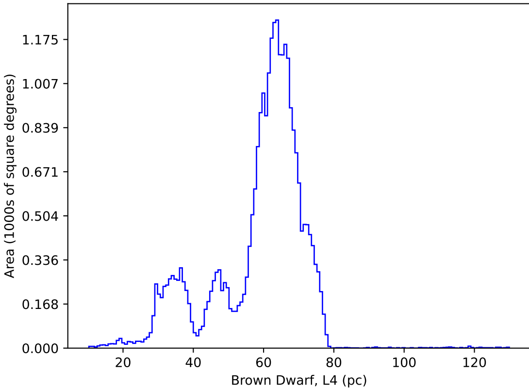
too_elab_r32_d2_griz_v3.4_10yrs : Brown Dwarf, L4
