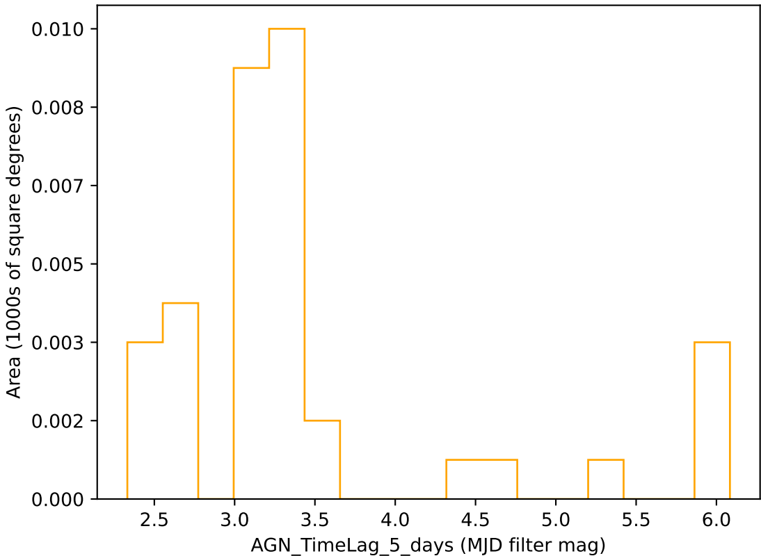
too_elab_r32_d2_griz_v3.4_10yrs r band: AGN_TimeLag_5_days
