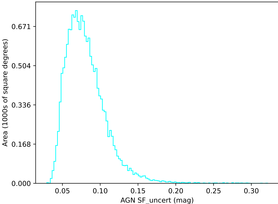
too_elab_r32_d2_griz_v3.4_10yrs u band: AGN SF_uncert
