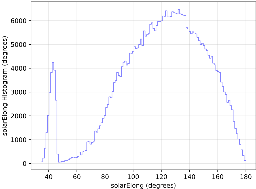
too_elab_r32_d2_griz_v3.4_10yrs WFD z band: solarElong Histogram
