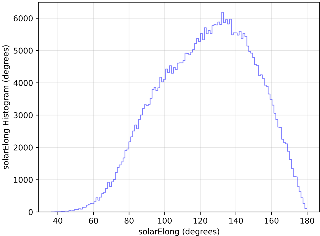
too_elab_r32_d2_griz_v3.4_10yrs WFD y band: solarElong Histogram
