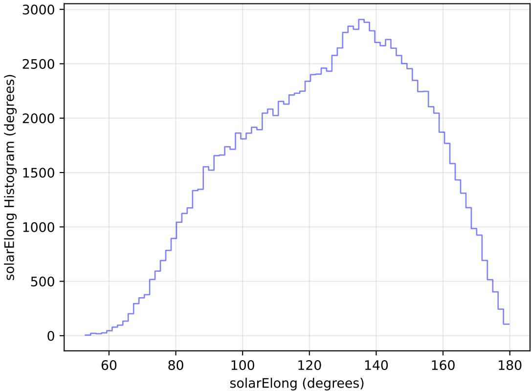
too_elab_r32_d2_griz_v3.4_10yrs WFD u band: solarElong Histogram
