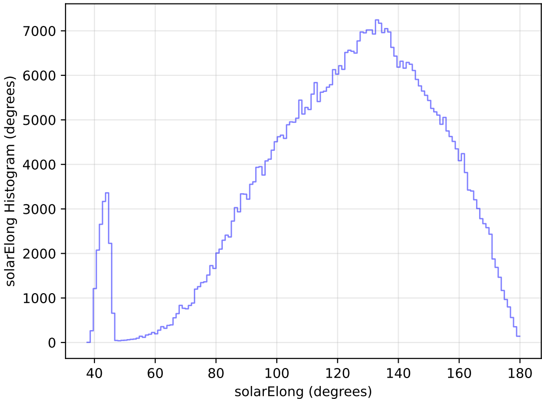
too_elab_r32_d2_griz_v3.4_10yrs WFD r band: solarElong Histogram
