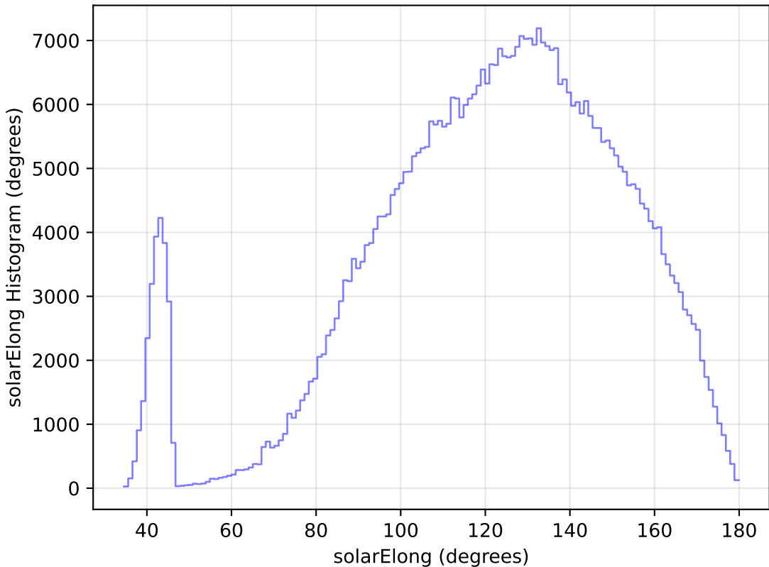
too_elab_r32_d2_griz_v3.4_10yrs WFD i band: solarElong Histogram
