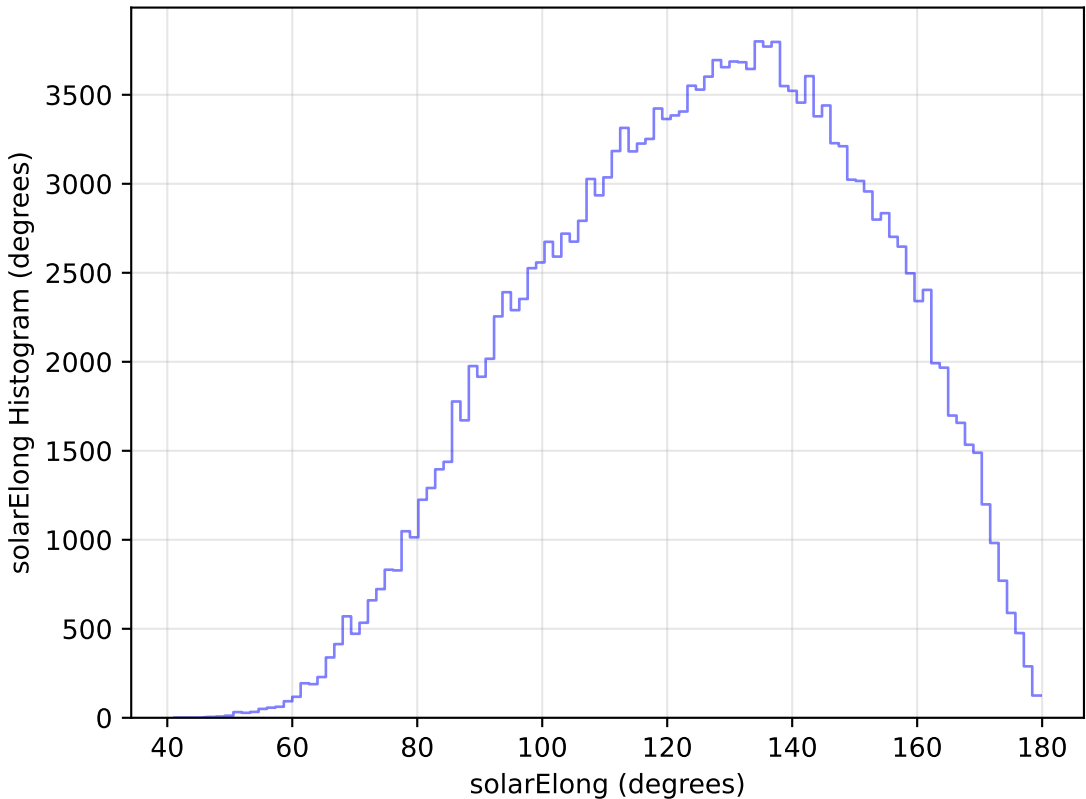
too_elab_r32_d2_griz_v3.4_10yrs WFD g band: solarElong Histogram
