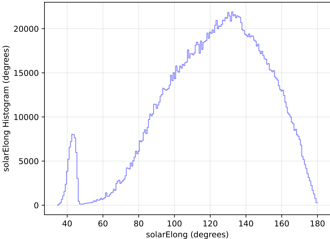
too_elab_r32_d2_griz_v3.4_10yrs WFD all bands: solarElong Histogram
