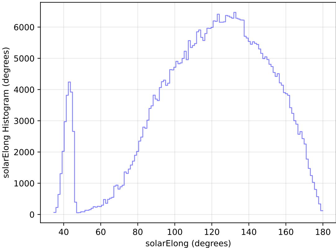
too_elab_r32_d2_griz_v3.4_10yrs All sky z band: solarElong Histogram
