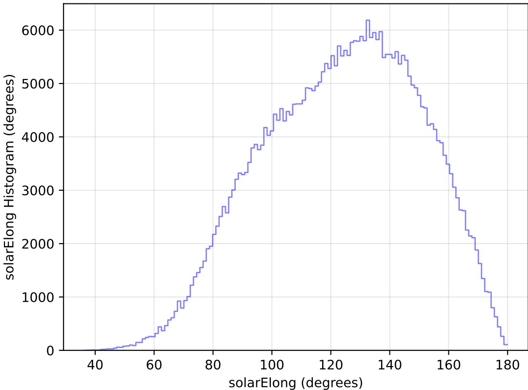
too_elab_r32_d2_griz_v3.4_10yrs All sky y band: solarElong Histogram
