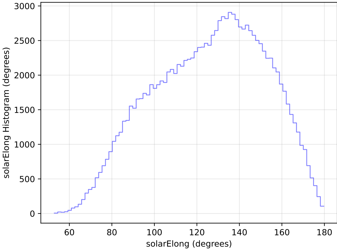
too_elab_r32_d2_griz_v3.4_10yrs All sky u band: solarElong Histogram
