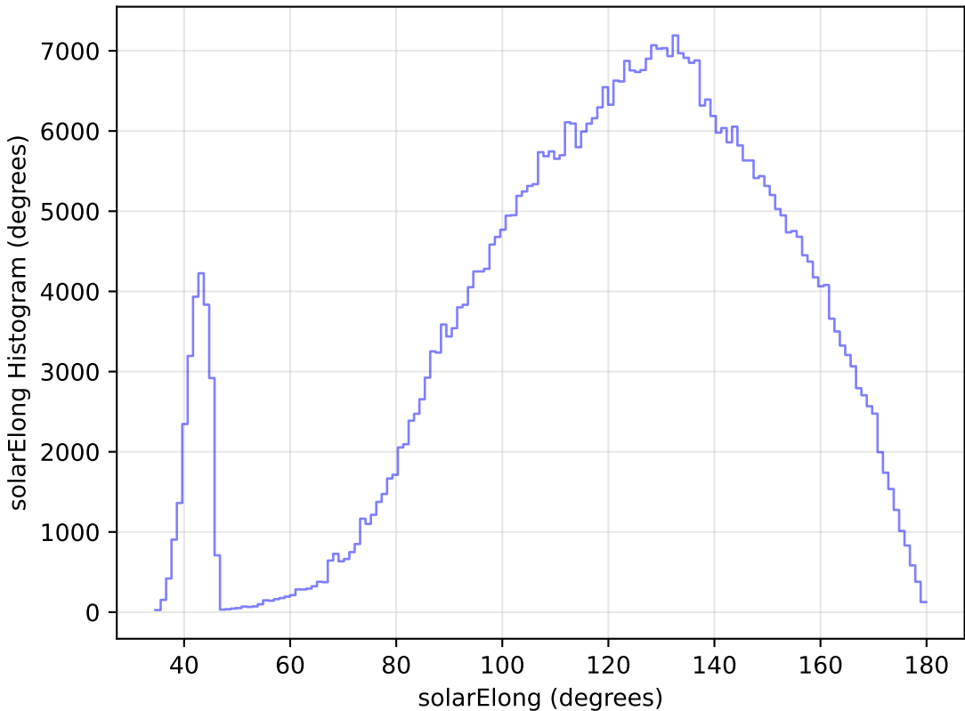
too_elab_r32_d2_griz_v3.4_10yrs All sky i band: solarElong Histogram
