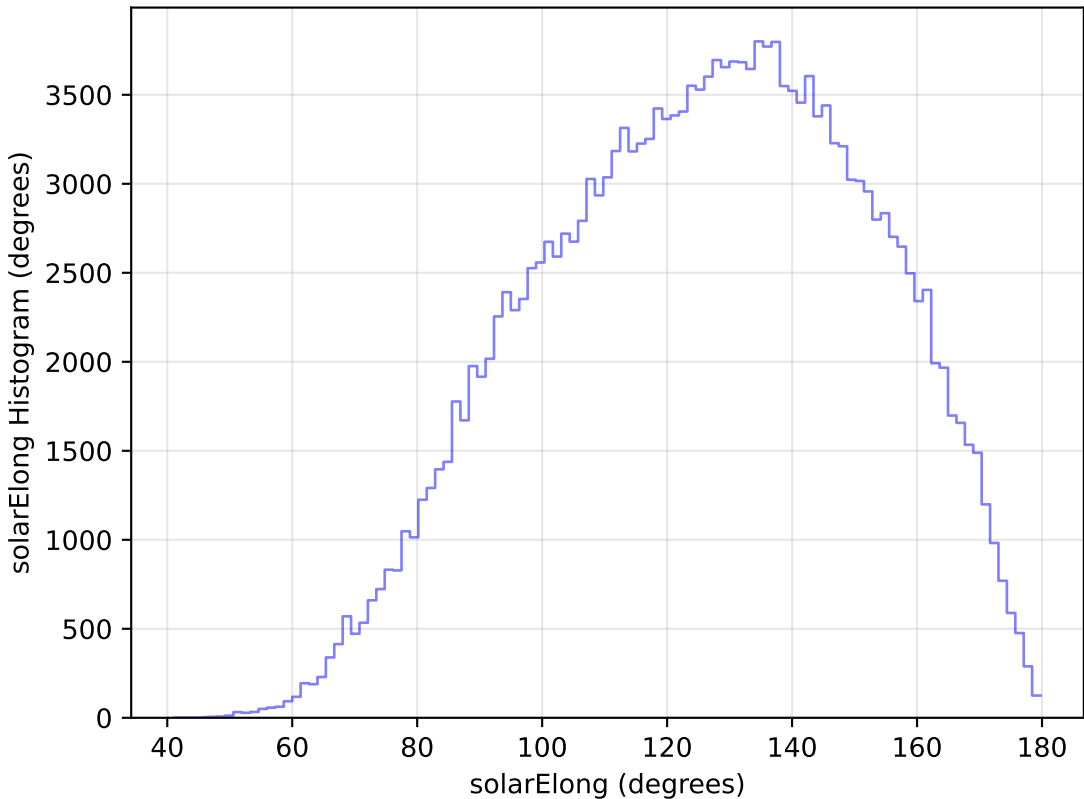
too_elab_r32_d2_griz_v3.4_10yrs All sky g band: solarElong Histogram
