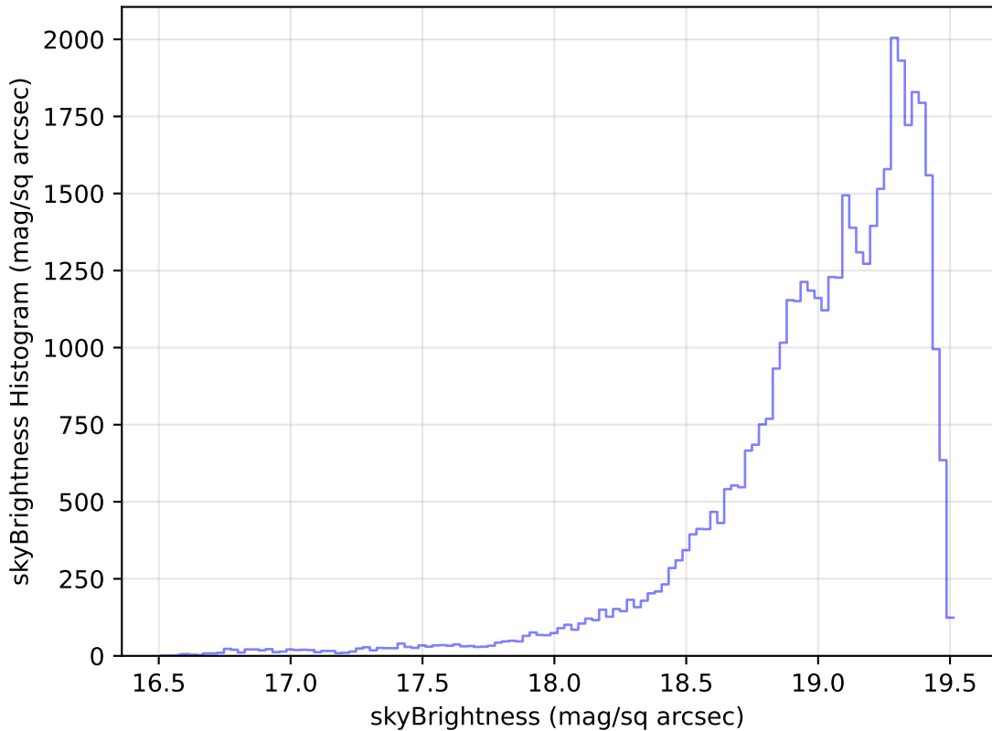
too_elab_r32_d2_griz_v3.4_10yrs Yr 1 z band: skyBrightness Histogram
