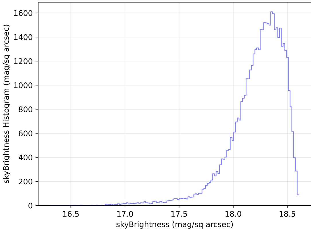
too_elab_r32_d2_griz_v3.4_10yrs Yr 1 y band: skyBrightness Histogram
