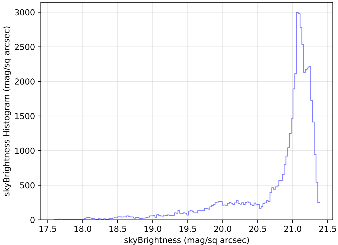
too_elab_r32_d2_griz_v3.4_10yrs Yr 1 r band: skyBrightness Histogram
