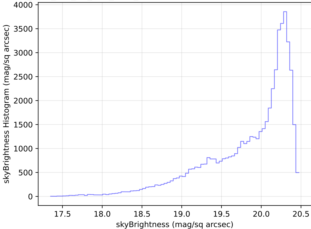
too_elab_r32_d2_griz_v3.4_10yrs Yr 1 i band: skyBrightness Histogram
