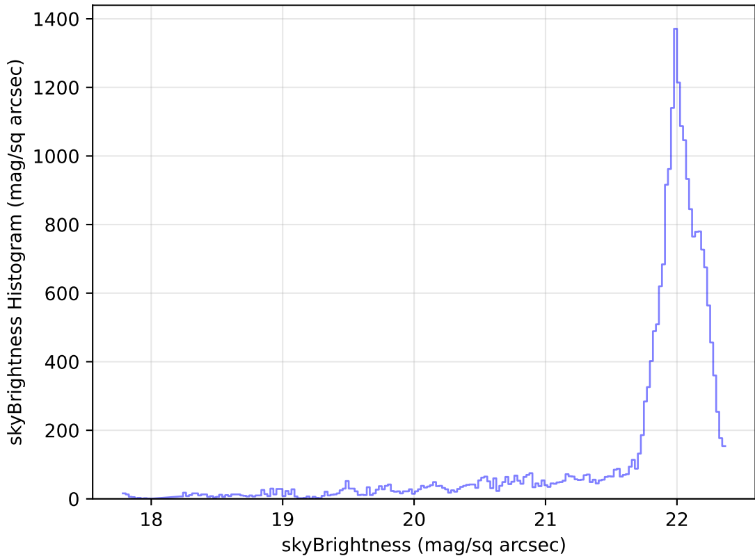
too_elab_r32_d2_griz_v3.4_10yrs Yr 1 g band: skyBrightness Histogram
