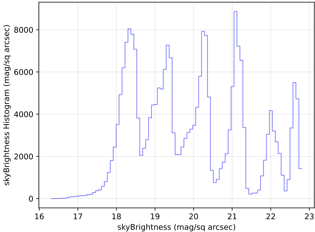
too_elab_r32_d2_griz_v3.4_10yrs Yr 1 all bands: skyBrightness Histogram
