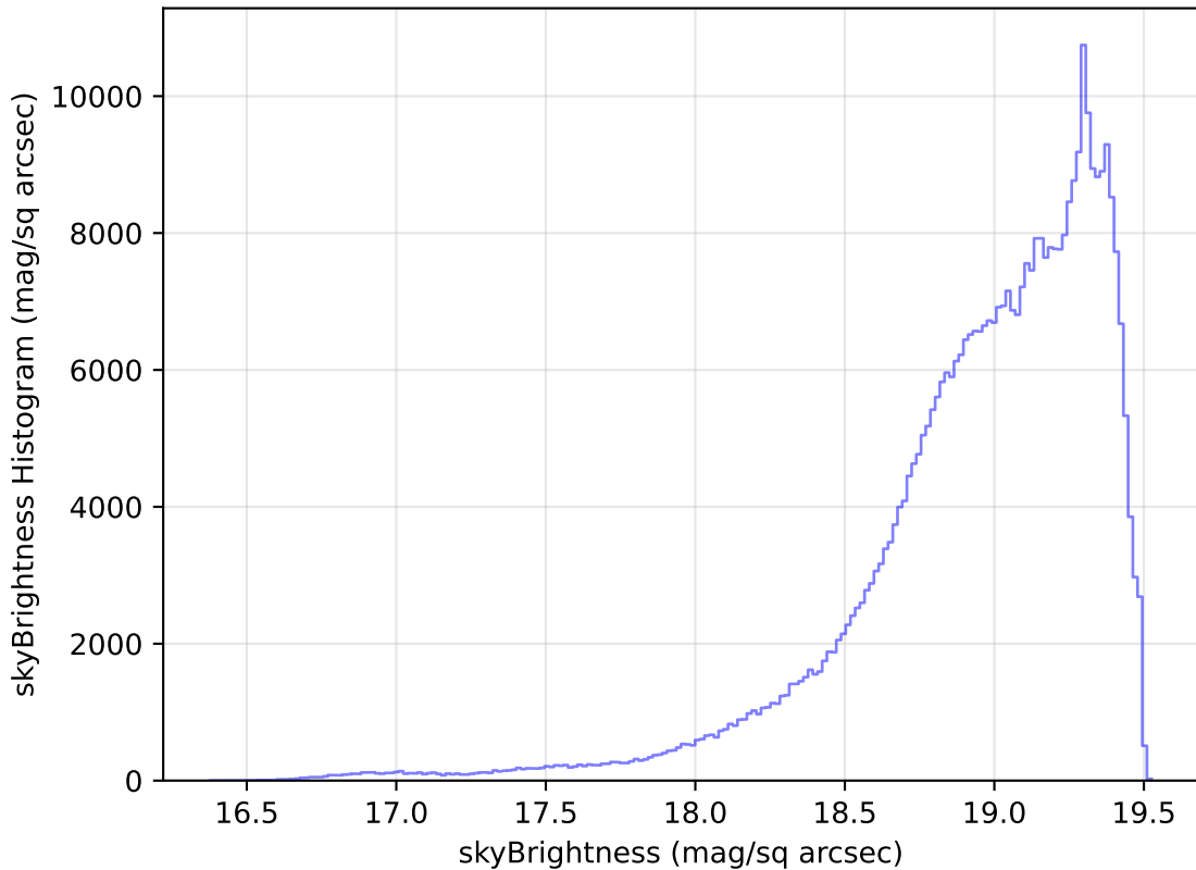
too_elab_r32_d2_griz_v3.4_10yrs WFD z band: skyBrightness Histogram
