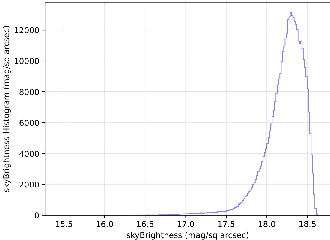
too_elab_r32_d2_griz_v3.4_10yrs WFD y band: skyBrightness Histogram
