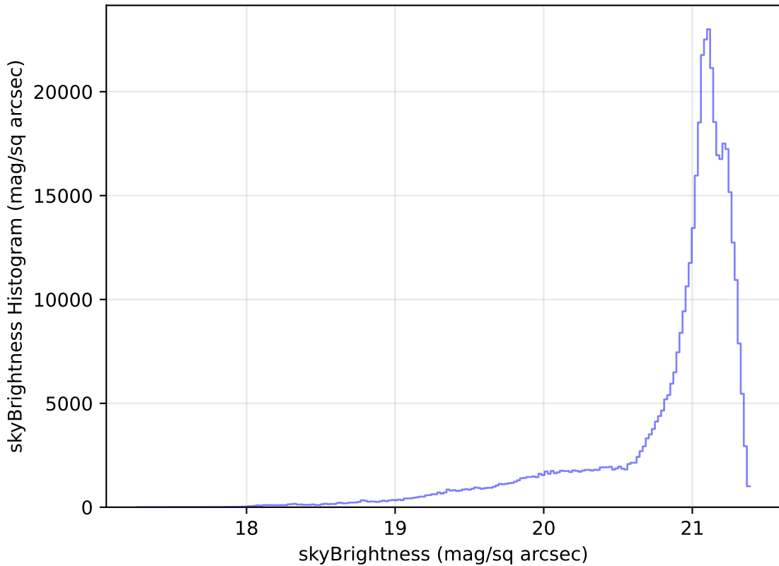
too_elab_r32_d2_griz_v3.4_10yrs WFD r band: skyBrightness Histogram
