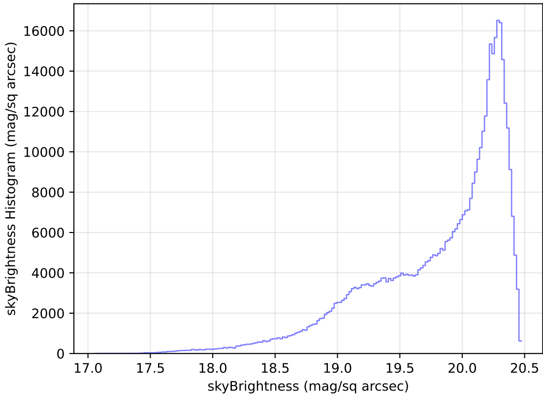
too_elab_r32_d2_griz_v3.4_10yrs WFD i band: skyBrightness Histogram
