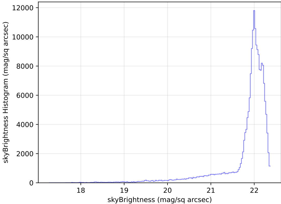
too_elab_r32_d2_griz_v3.4_10yrs WFD g band: skyBrightness Histogram
