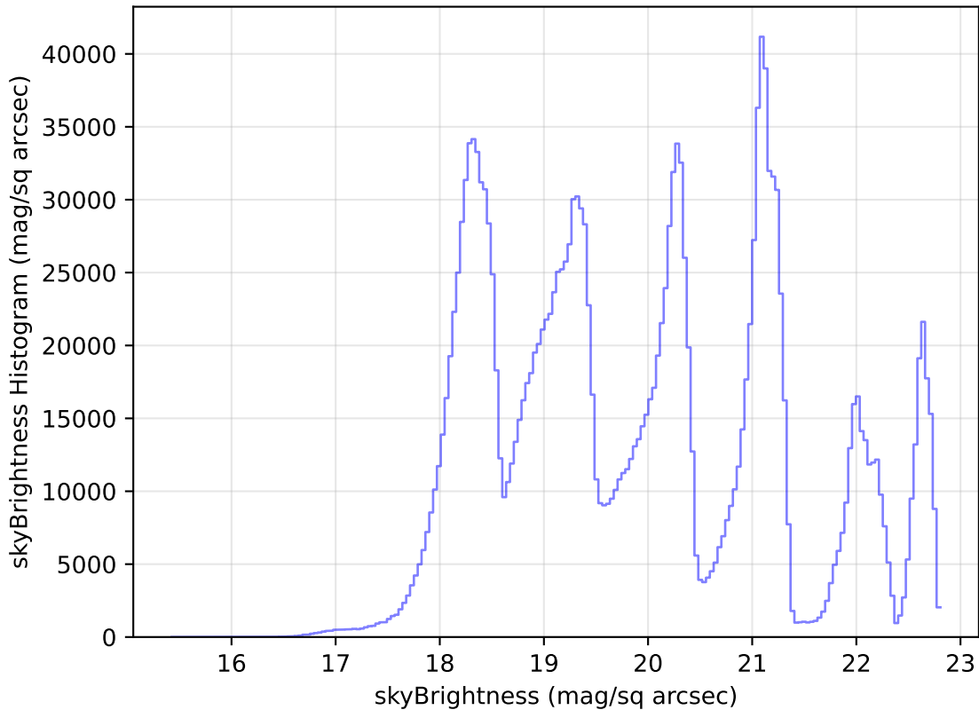
too_elab_r32_d2_griz_v3.4_10yrs WFD all bands: skyBrightness Histogram
