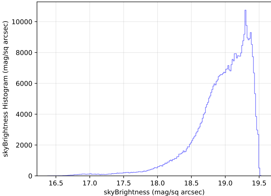
too_elab_r32_d2_griz_v3.4_10yrs All sky z band: skyBrightness Histogram
