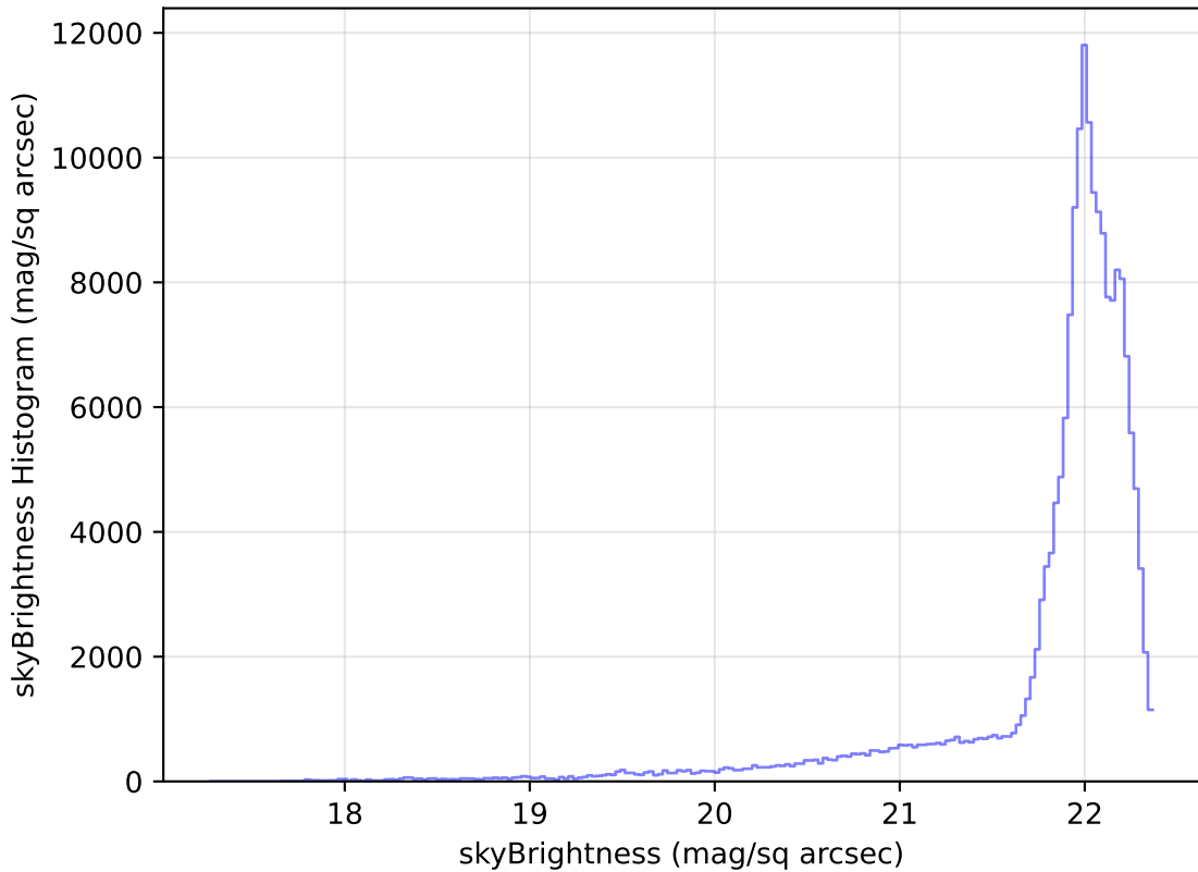
too_elab_r32_d2_griz_v3.4_10yrs All sky g band: skyBrightness Histogram
