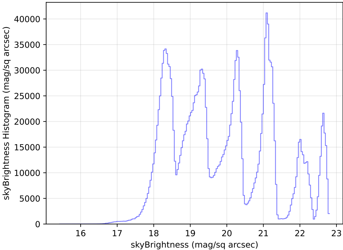
too_elab_r32_d2_griz_v3.4_10yrs All sky all bands: skyBrightness Histogram
