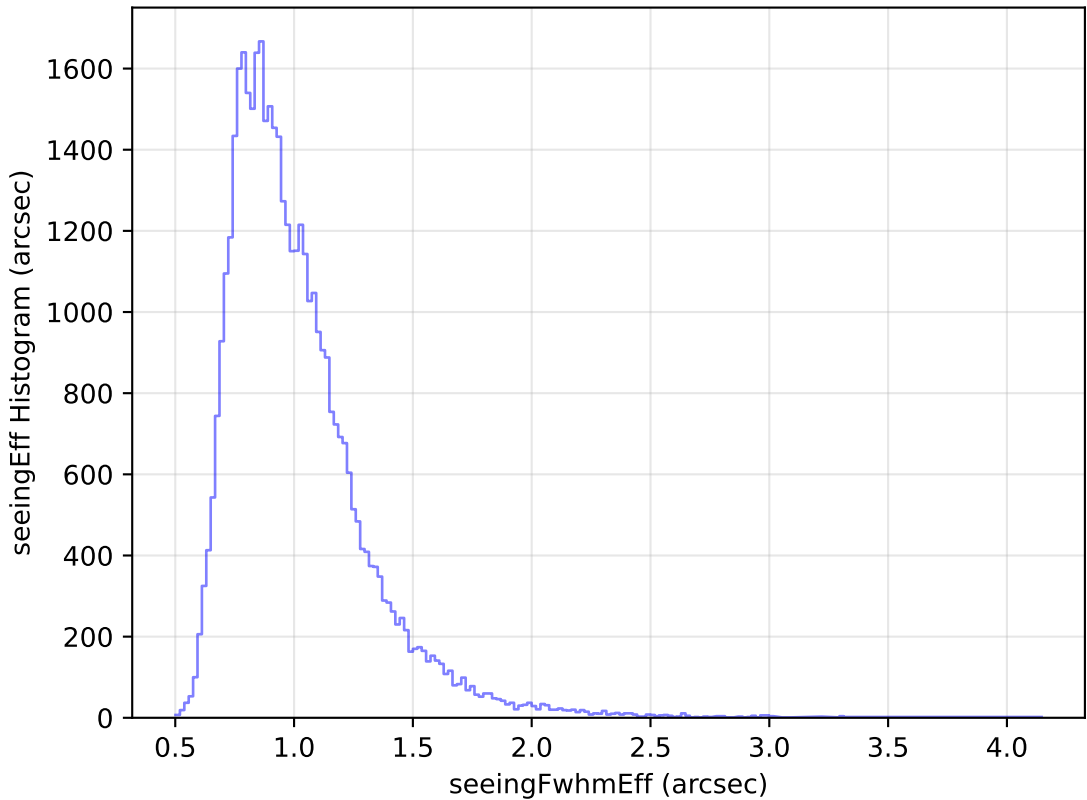
too_elab_r32_d2_griz_v3.4_10yrs Yr 1 z band: seeingEff Histogram
