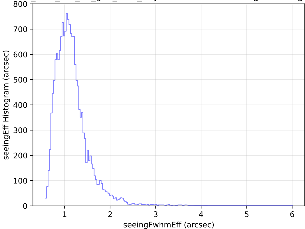
too_elab_r32_d2_griz_v3.4_10yrs Yr 1 u band: seeingEff Histogram
