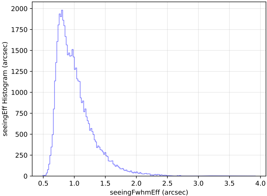
too_elab_r32_d2_griz_v3.4_10yrs Yr 1 r band: seeingEff Histogram
