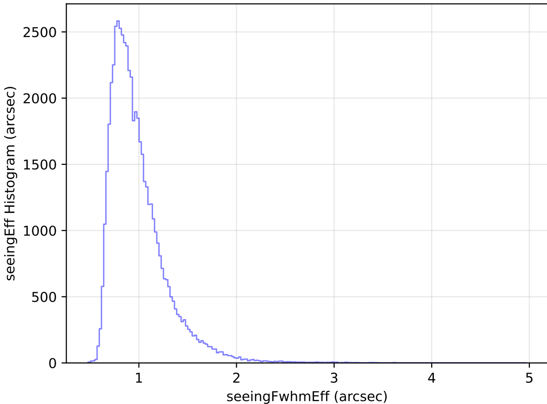
too_elab_r32_d2_griz_v3.4_10yrs Yr 1 i band: seeingEff Histogram
